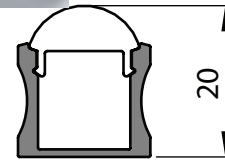
with optic lens 30° SCALE 1:1 (A4)
